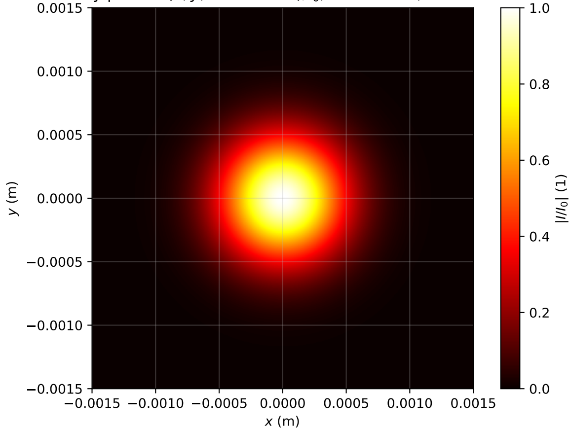
Intensity profile I(x, y, z = 0.080\text{m})/I_0 , Pin=0.3Pcr, artificial time
